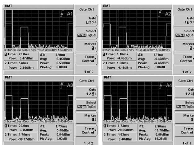
Figure 7. Measurement flexibility with 4 independent time gates
